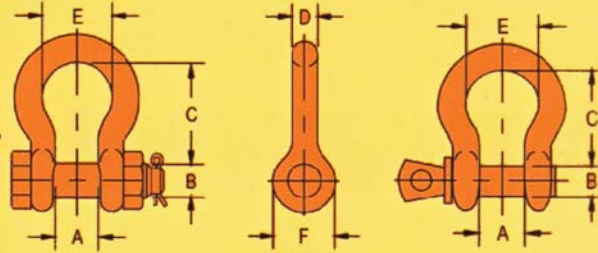
HOT DIP GALV'D SHACKLE (SCREW PIN & BOLT & NUT)
